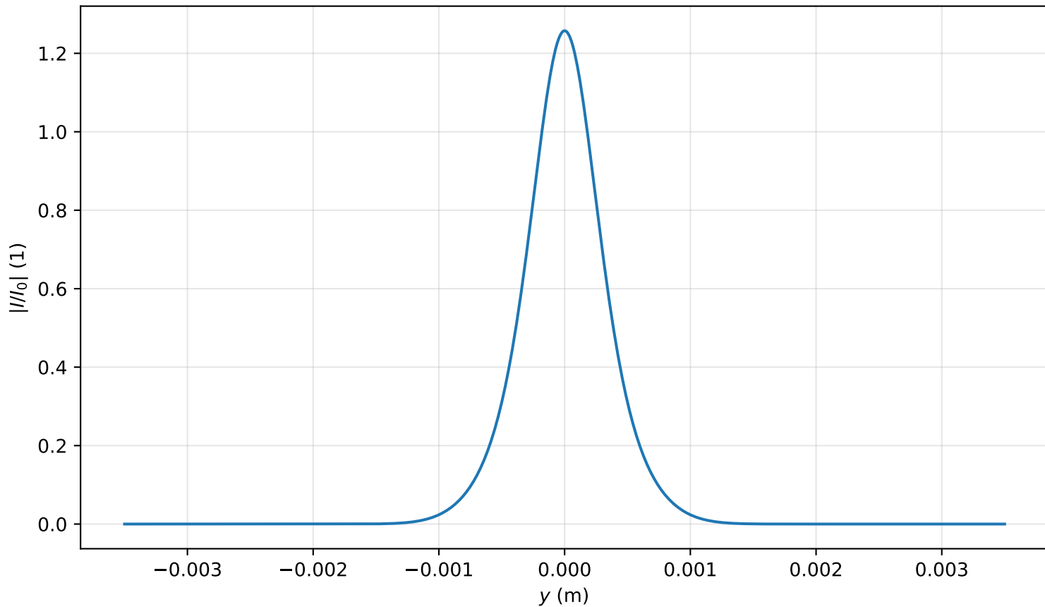
Intensity profile I(x=0, y, z=0.876)/I_0 , P_{in}=0.8P_{cr} , artificial time
